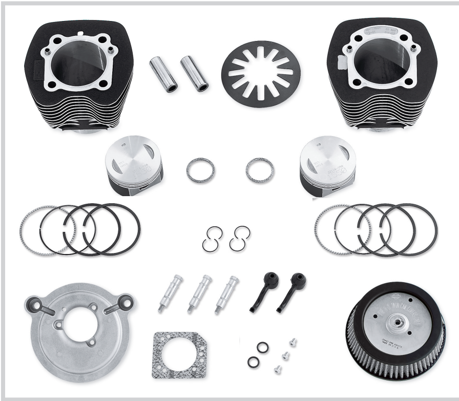
SCREAMIN' EAGLE® BIG BORE STAGE I KIT FOR EFI MODELS – 103 CUBIC INCHES
