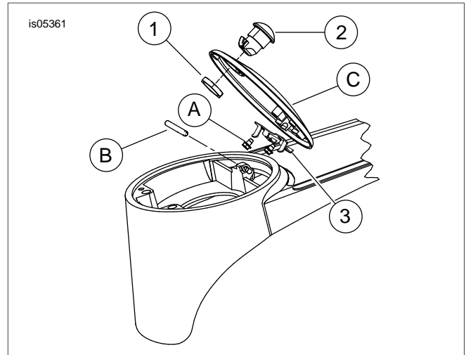
Figure 1. Service Parts: Console Pushbutton Fuel Door Release
