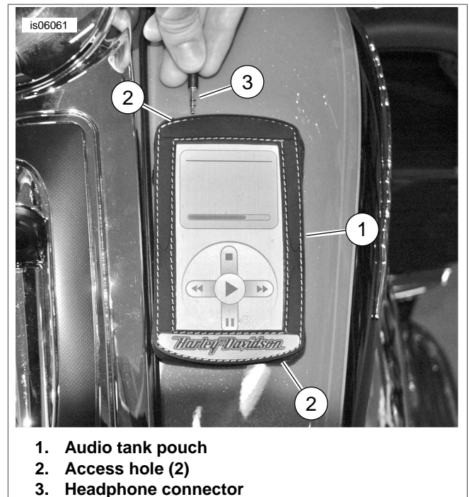
Figure 2. Audio Tank Pouch on Fuel Tank
