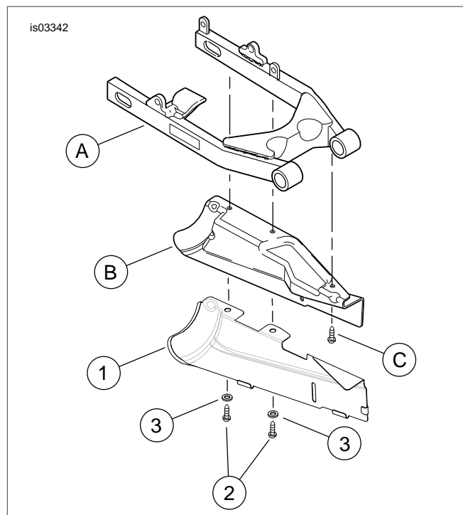
Figure 1. Service Parts: Chrome Debris Deflector Cover
