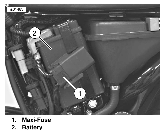
Figure 1. Disconnect Maxi-Fuse
