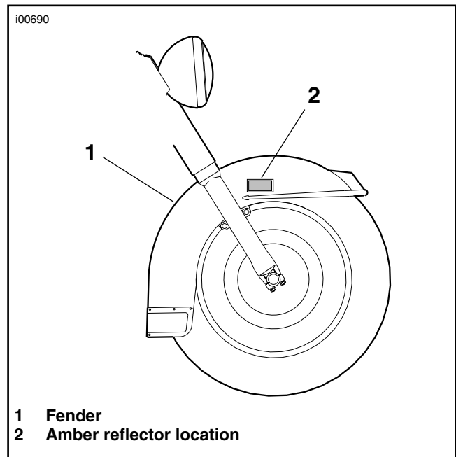
Figure 1. Mounting Amber Reflectors
