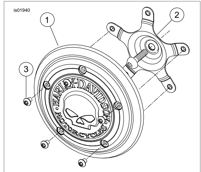
Figure 1. Service Parts: Skull Air Cleaner Cover Shown
