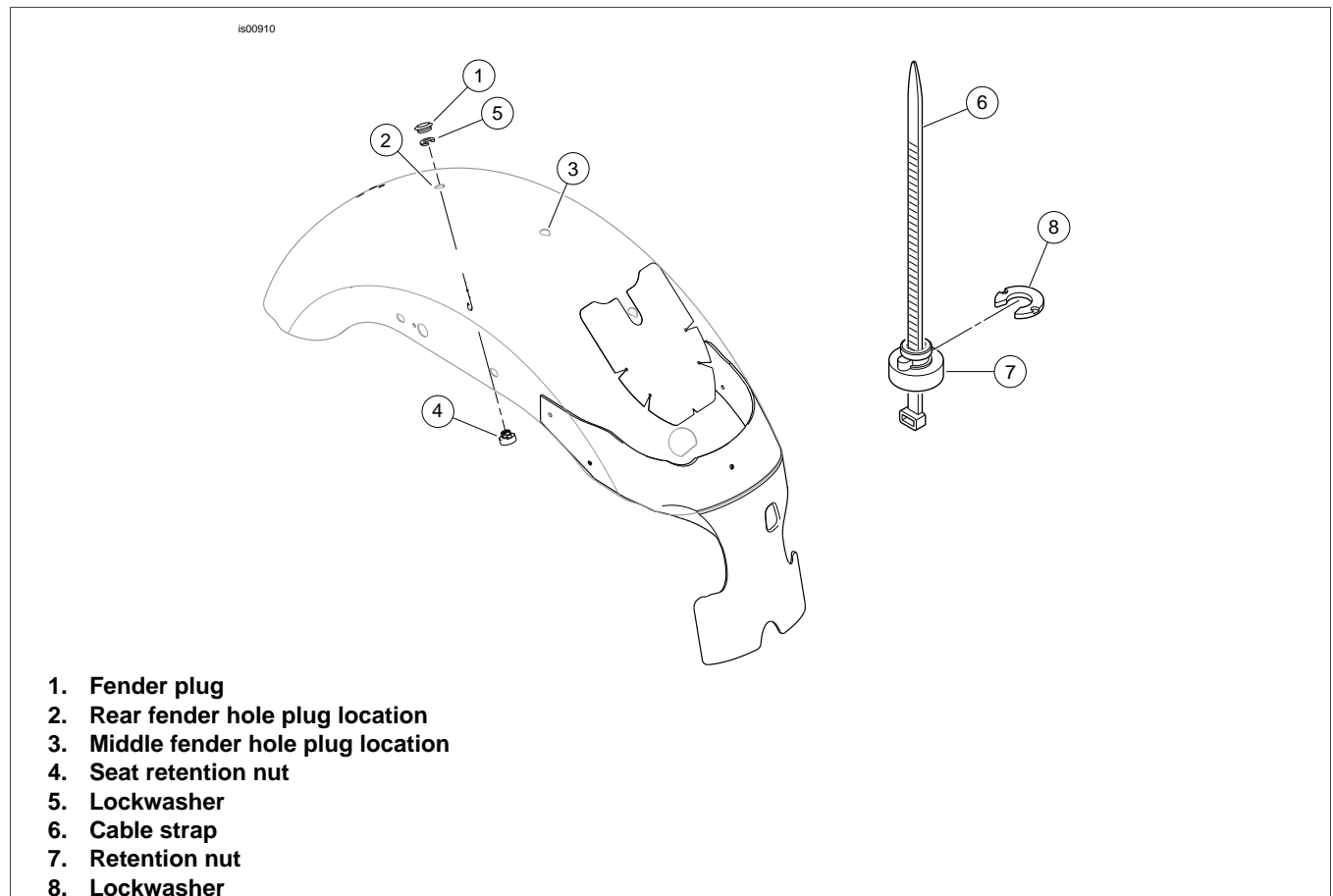
Figure 1. Fender Hole Locations
